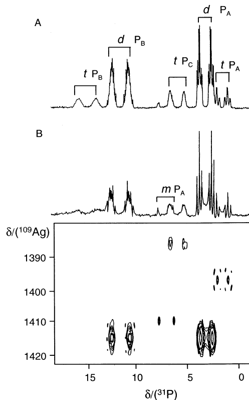
Fig. 2. The normal ^{31}\text{P}\{-^1\text{H}\} -NMR spectrum of a solution of \{[\text{Ag}(\text{d2pype})_2]\text{NO}_3\}_n at 243 K (A), and the [^{31}\text{P}, ^{109}\text{Ag}] spectrum in \text{CD}_3\text{OD} at the same temperature (B) (see Fig. 1 for assignments). (Adapted from Ref. [31]).
